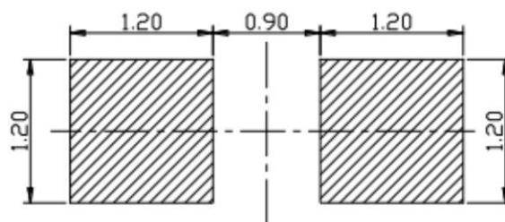
推荐焊盘尺寸 Recommended Soldering Pad
