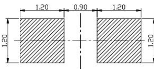
推荐焊盘尺寸 Recommended Soldering Pad
