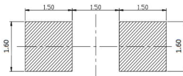
推荐焊盘尺寸 Recommended Soldering Pad
