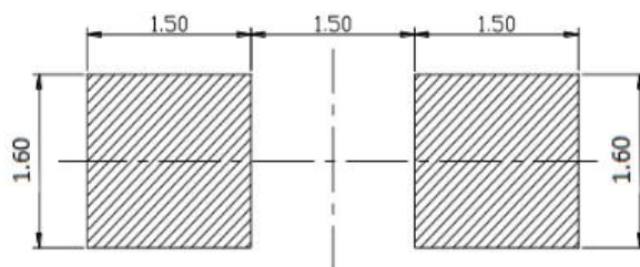
推荐焊盘尺寸 Recommended Soldering Pad
