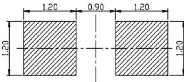
推荐焊盘尺寸 Recommended Soldering Pad
